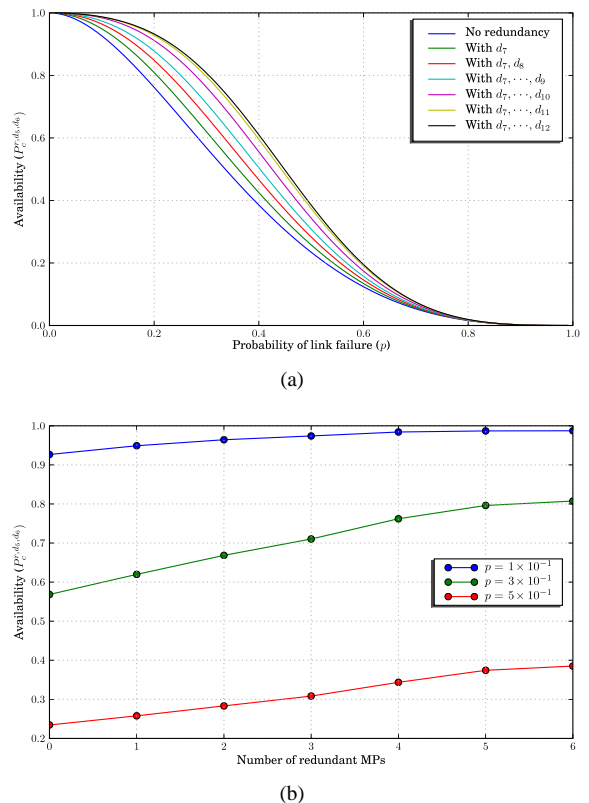
Figure 4. The availability depends on (a) the link failure probability p , and (b) the number of redundant nodes.
