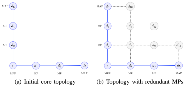
Figure 3. Topology with or without redundant MPs
