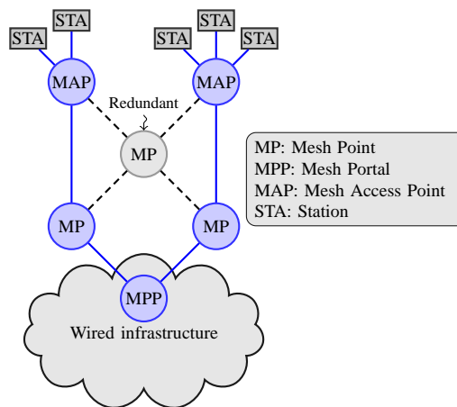
Figure 1. A backhaul mesh network with a redundant node.
