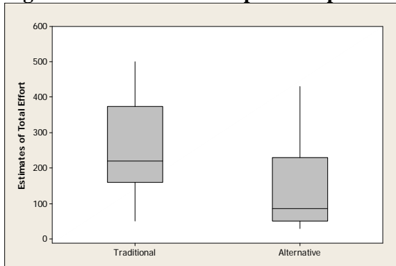
Figure 2: Effort Estimates per Group
